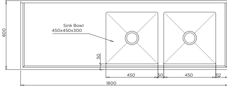
MODEL BT-DSB-618-R Plan
