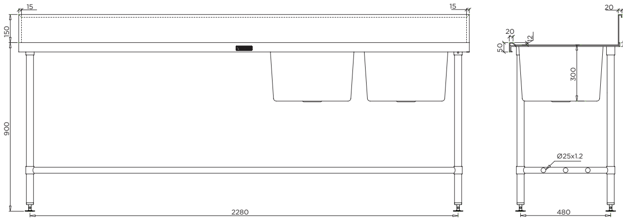
MODEL BT-DSB-624-R Front Elevation and Section
