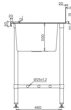
MODEL BT-DSB-618-R Section
