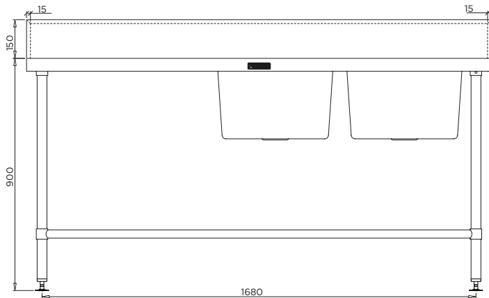
MODEL BT-DSB-618-R Front Elevation
